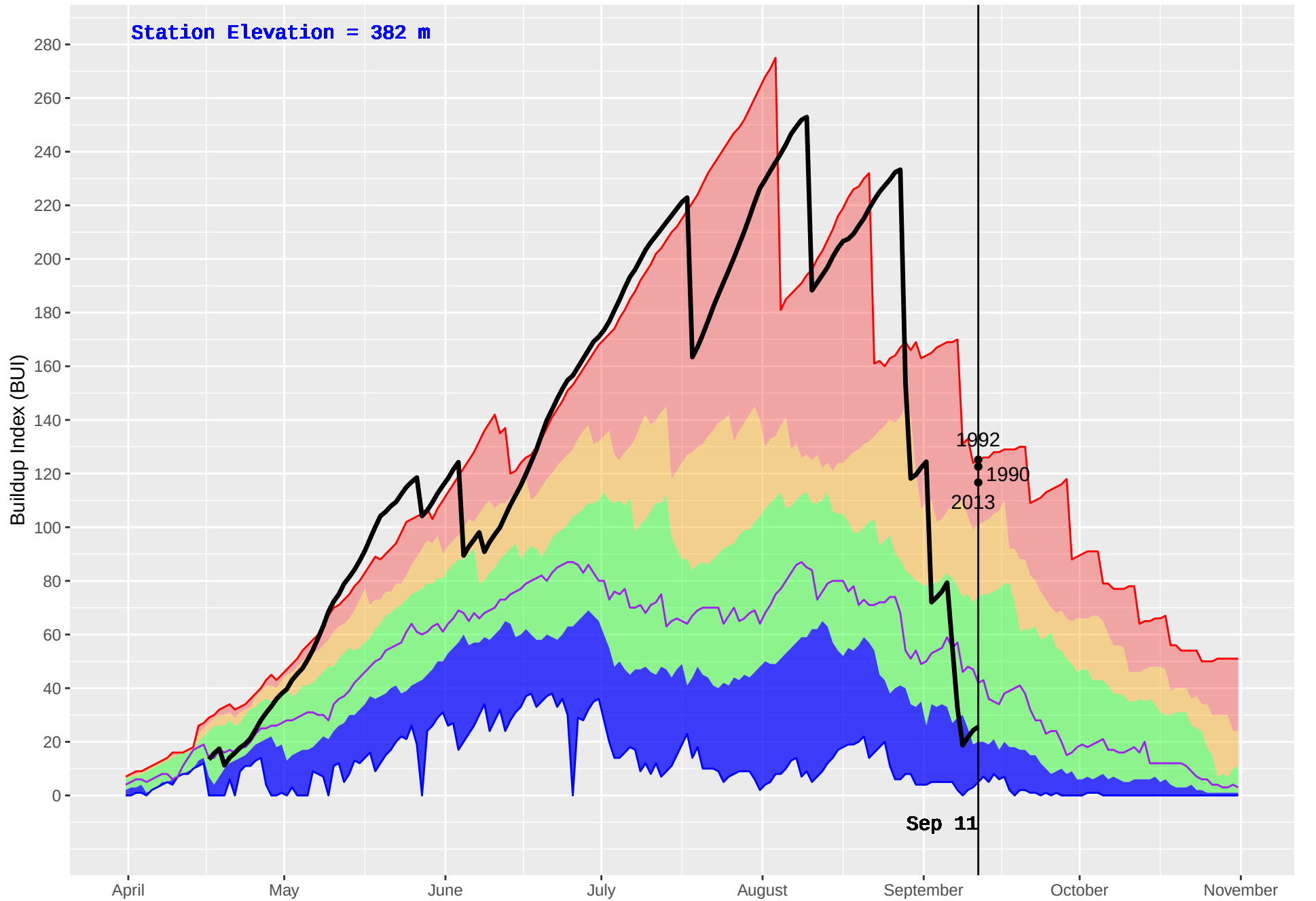
TELEGRAPH CREEK (110) : Historical (1978–2016) and Current (2018) Daily Buildup Index (BUI)
